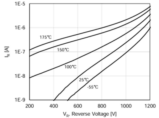
Figure 4. Reverse Characteristics
