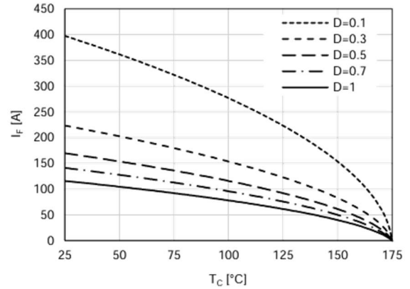
Figure 2. Current Derating
