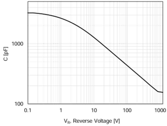
Figure 7. Capacitance Characteristics
