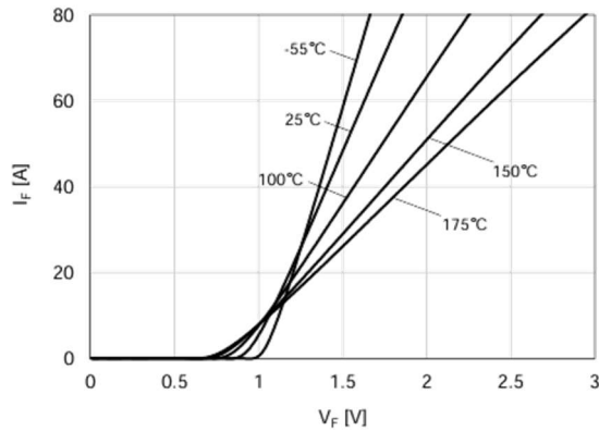
Figure 3. Forward Characteristics
