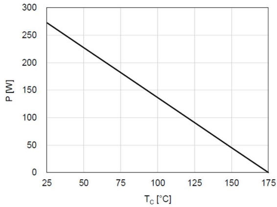
Figure 1. Power Derating
