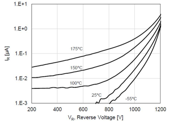
Figure 4. Reverse Characteristics
