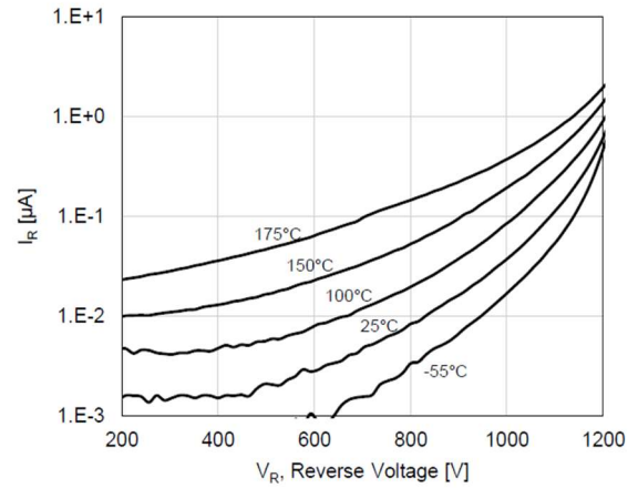
Figure 4. Reverse Characteristics
