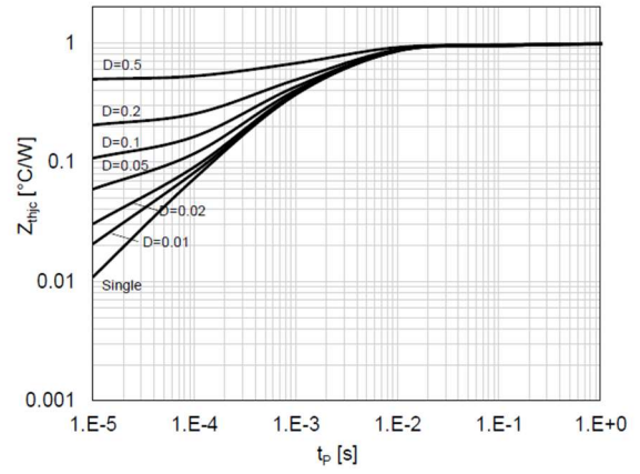
Figure 8. Transient Thermal Response Curve
