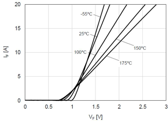
Figure 3. Forward Characteristics
