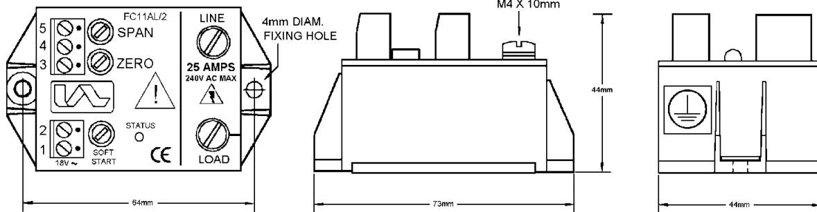
SIDE VIEW POWER CONNECTIONS M4 X 10mm
