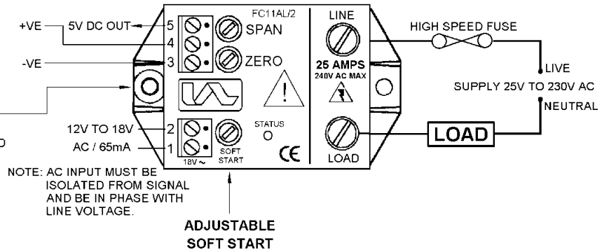
SIDE VIEW POWER CONNECTIONS M4 X 10mm
